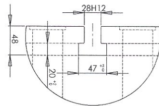
DETAIL C SCALE 1 : 3
